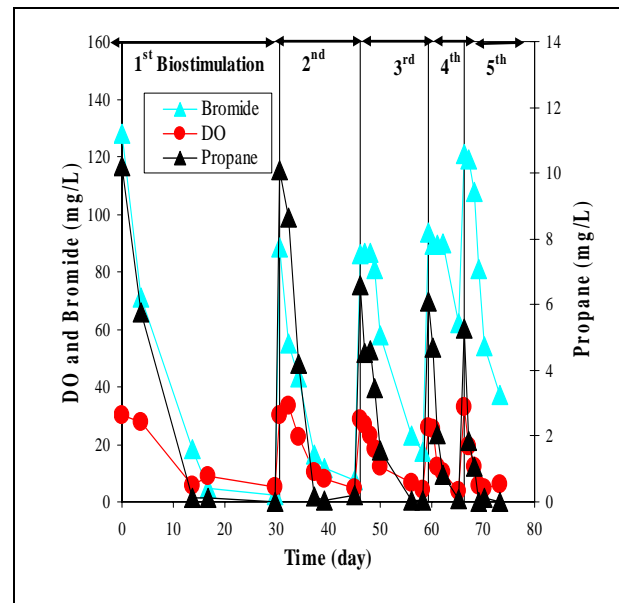
Figure 5. Measured Propane, Oxygen, and Bromide Concentrations During Five Field Biostimulation Tests Conducted at the McAFB, California (MW2) Field.
